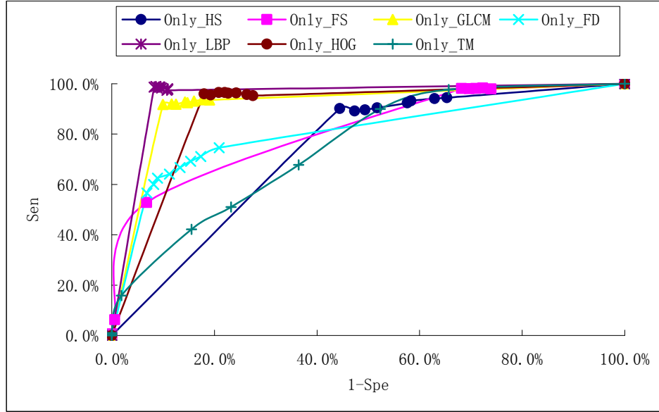
Fig. 5.5. ROC curves of different features using SVM.
