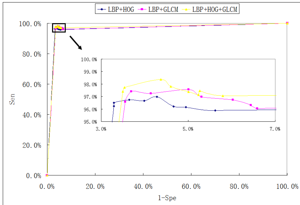
Fig. 5.8. ROC curves using different combination of LBP, GLCM and HOG features with Adaboost. To better discriminate different curves, the rectangle area has been enlarged and shown in the middle.
