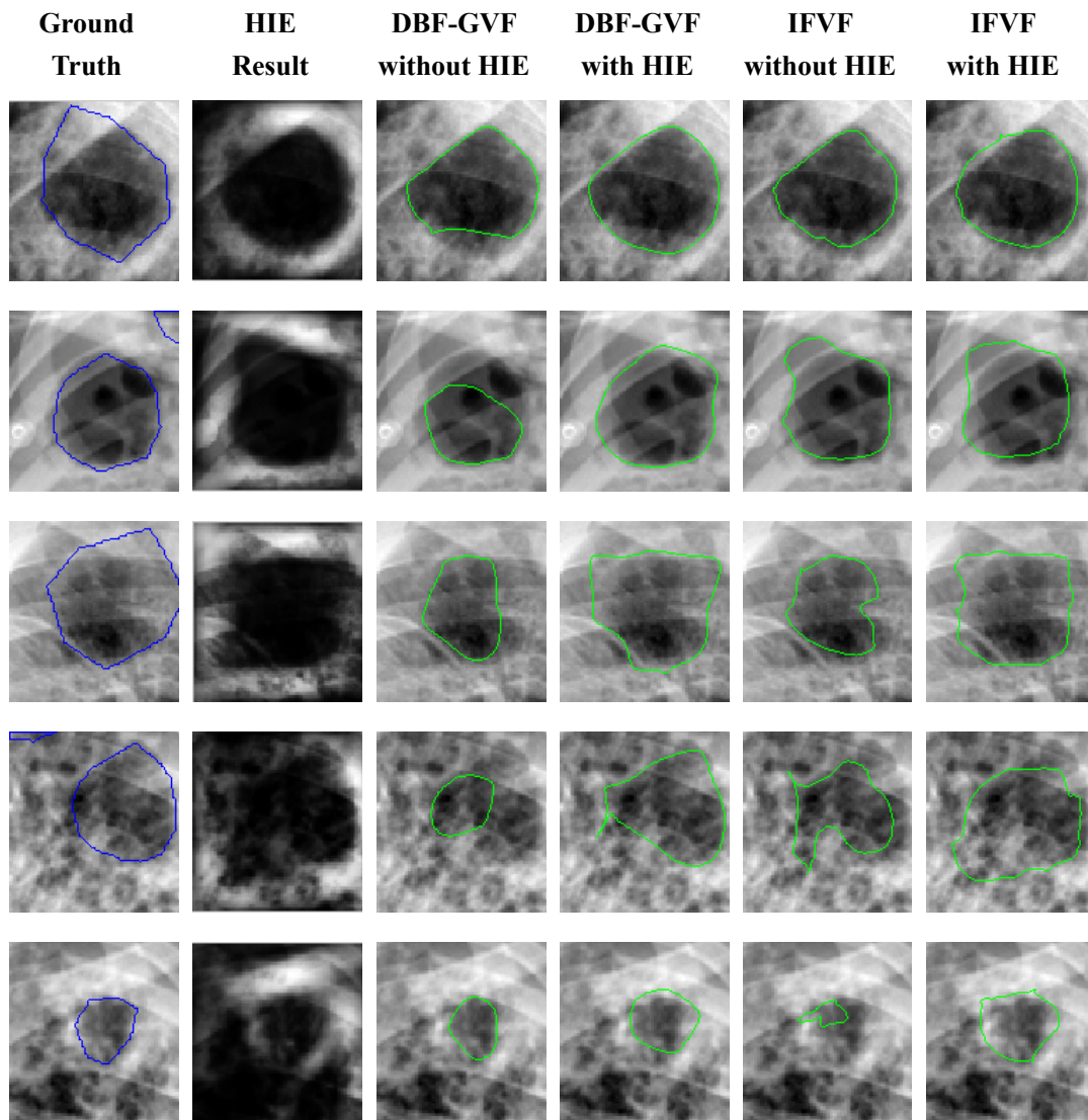
Fig. 4.12. Cavity segmentation result comparison using different edge-based snakes with and without HIE. From top to bottom, the cavity is more and more difficult to identify. Blue contours are the true cavities annotated by radiologists. Green contours are the computer segmentation results.
