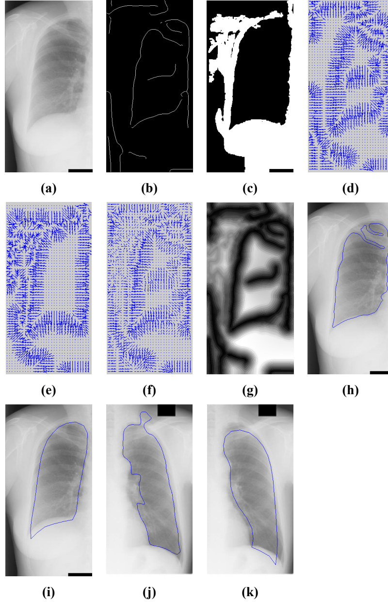
Fig. 3.2. An example of our automatic initialization using edge and region force fields: (a) The original right half lung image; (b) Optimized edge map B ; (c) Optimized region map R ; (d) Diffused edge force field f_E ; (e) Diffused region force field f_R ; (f) Total ERF field f_{ERF} ; (g) Estimated energy field of the force f_{ERF} ; (h) PIG-based initialization; (i) Our initialization. Another comparison is shown in (j) PIG-based initialization and (k) our initialization.
