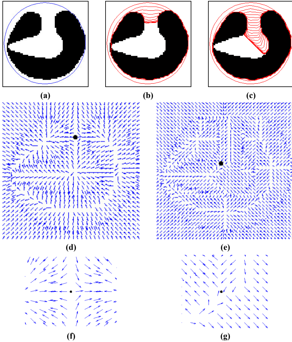
Fig. 2.4. Stationary or saddle point examples in GVF and BVF. (a) Acute concave shape with an initial contour as a blue circle; (b) Segmentation result using GVF; (c) Segmentation result using BVF; (d) Stationary point in GVF; (e) Saddle point in BVF; (f) GVF force field of the local area containing stationary point (the black point); (g) BVF force field of the local area containing saddle point.
