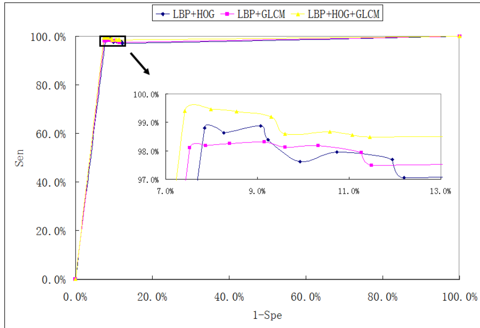
Fig. 5.7. ROC curves using different combination of LBP, GLCM and HOG features with SVM. To better discriminate different curves, the rectangle area has been enlarged and shown in the middle.
