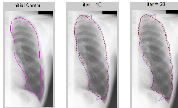
Fig. 3.5. 2-D points evolution using PEE (3.6) with w=1 , p=20 , q=1 (solid line) and PEE (3.7) with w=1 (dotted line). The points evolution using PEE (3.6) jumps to some false edges at iteration time t = 10 and 20 comparing to the more accurate points evolution result of PEE (3.7).
