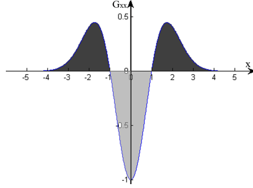
Fig. 4.7. The 2 nd derivative of a 1D Gaussian kernel probes inside/outside contrast of the range (-\sigma, \sigma) . In this example, G_{xx}(x) = (\frac{x^2}{\sigma^4} - \frac{1}{\sigma^2})e^{-\frac{x^2}{2\sigma^2}} , \sigma=1 .
