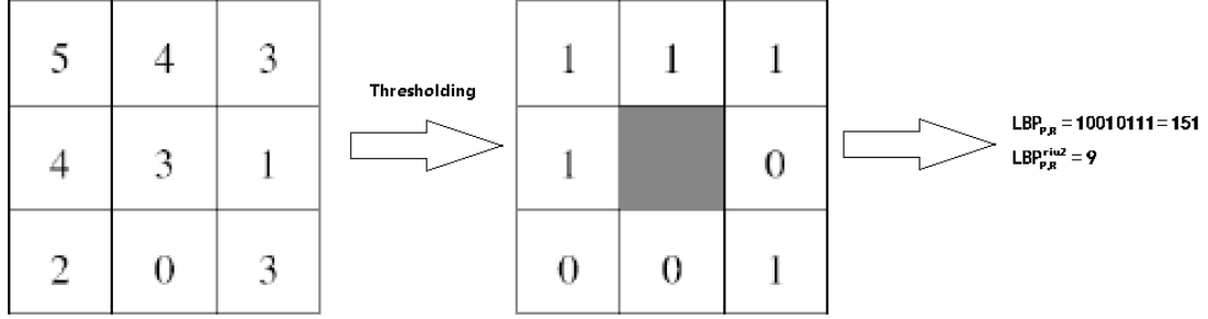
Fig. 2.8. An example of calculating LBP values in a 3×3 neighborhood.
