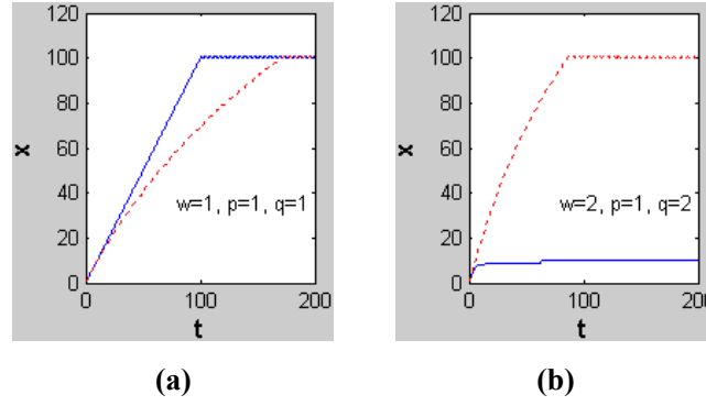
Fig. 3.3. Example of 1-D point evolution using PEE (3.6) (solid line) and PEE (3.7) (dotted line). While both converging to the strong edges in graph (a), the point evolution by using PEE (3.6) fails in graph (b) showing that it is sensitive to even a small change in the parameter values.
