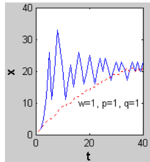
Fig. 3.4. Another example of 1-D point evolution using PEE (3.6) (solid line) and PEE (3.7) (dotted line). When changes are more rapid in a 1-D GVF field, point evolution using PEE (3.6) has strong ring effect while the result of PEE (3.7) appears more stable.
