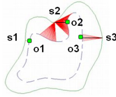
Fig. 4.8. An example of control point selection. s1-s3, o1-o3 are points on the snake contour and object boundary, respectively.
