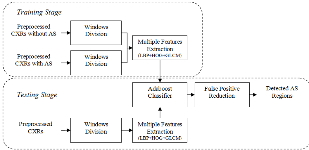
Fig. 5.2. Schematic of the proposed CAD system for AS detection.
