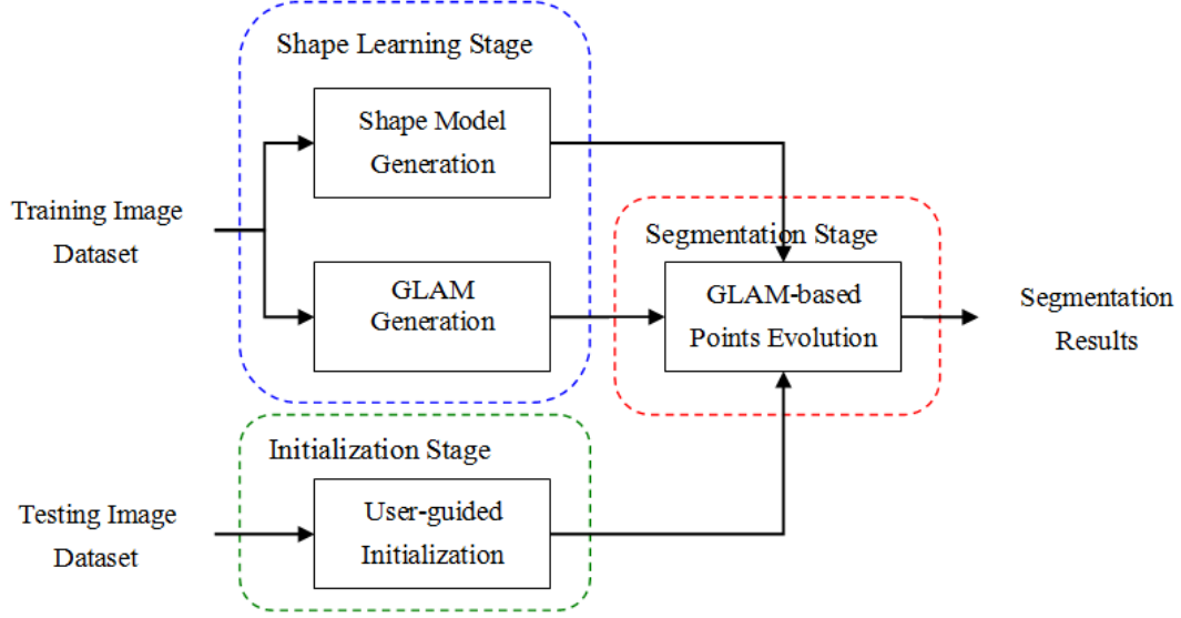
Fig. 2.1. Schematic of a typical ASM segmentation method.
