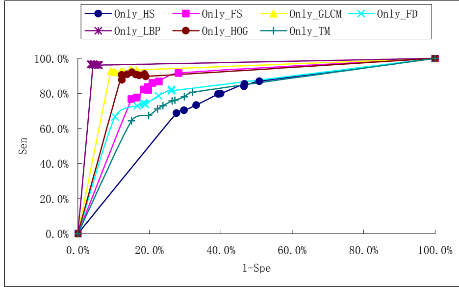
Fig. 5.6. ROC curves of different features using Adaboost.
