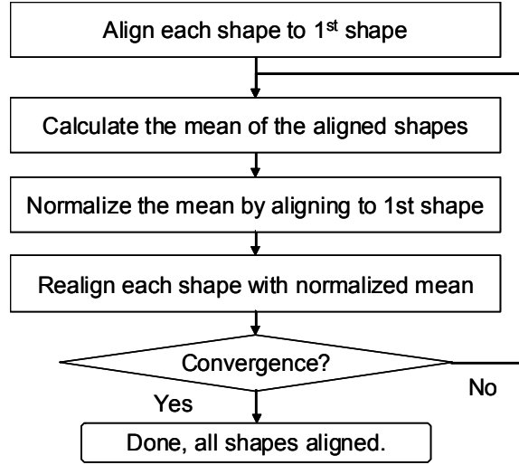
Fig. A.1 The flow diagram of the generalized Procrustes analysis.
