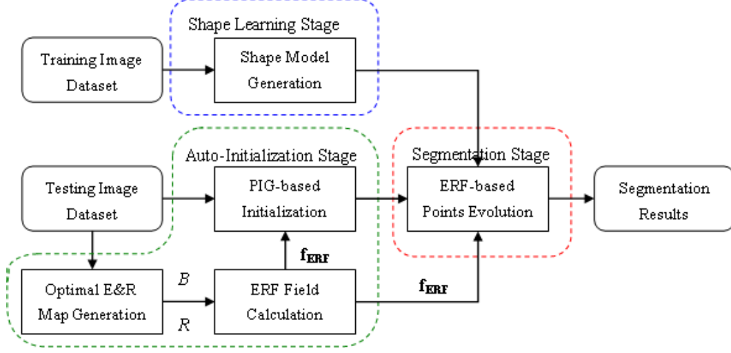
Fig. 3.1. Schematic of our proposed ERF-ASM for automatic lung field segmentation.
