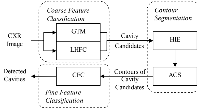
Fig. 4.2. Schematic of the proposed CAD framework.
