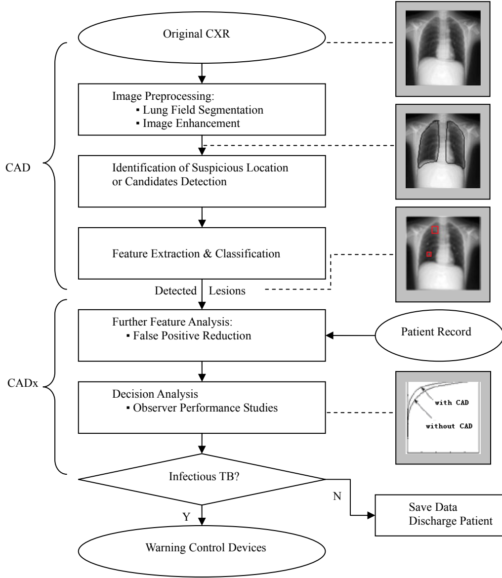
Fig. 1.4. Conceptual framework of the intelligent CAD system.
