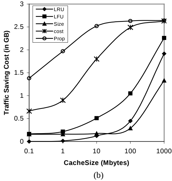
Figure 4.5 Traffic saving cost versus cache size. a) trace1, and b) trace2.
