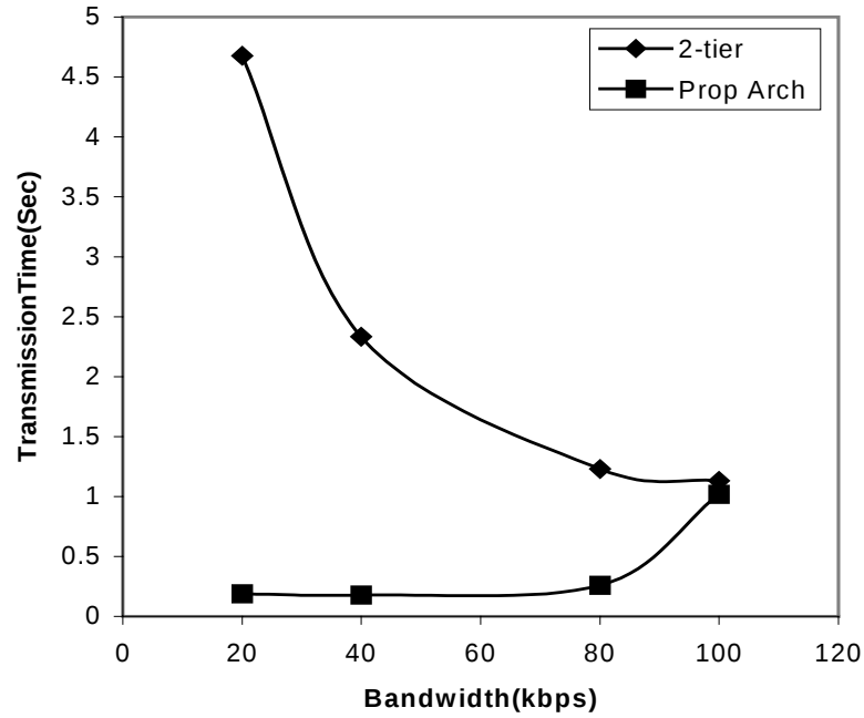
Figure 4.15 Performance of proposed architecture when compared with a 2-tier architecture
