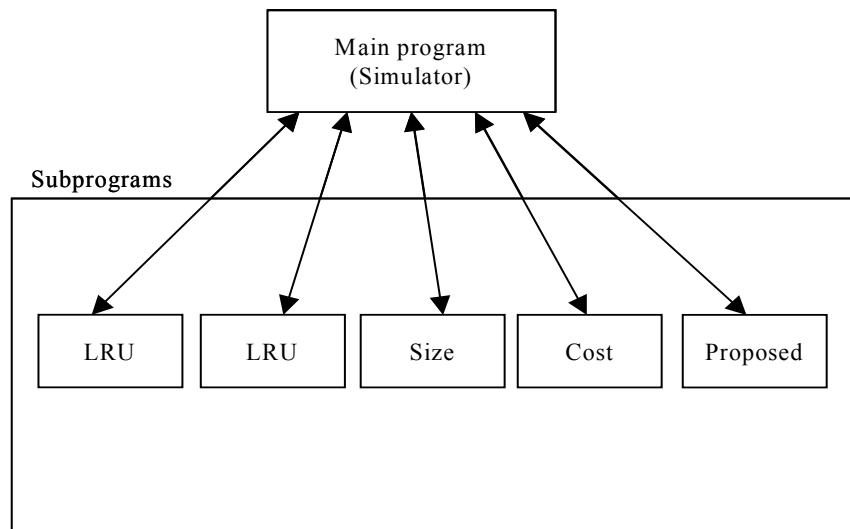
Figure A.2 Façade design pattern used by the trace driven simulator
