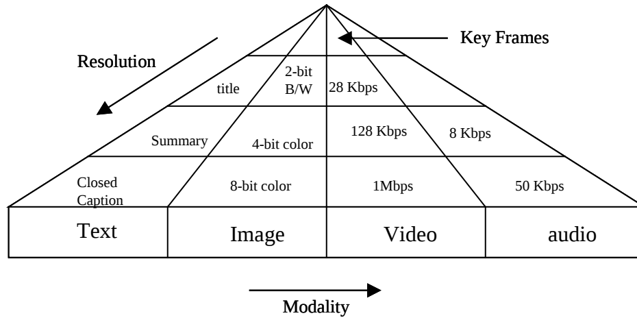
Figure 2.3 InfoPyramid scheme [3]
