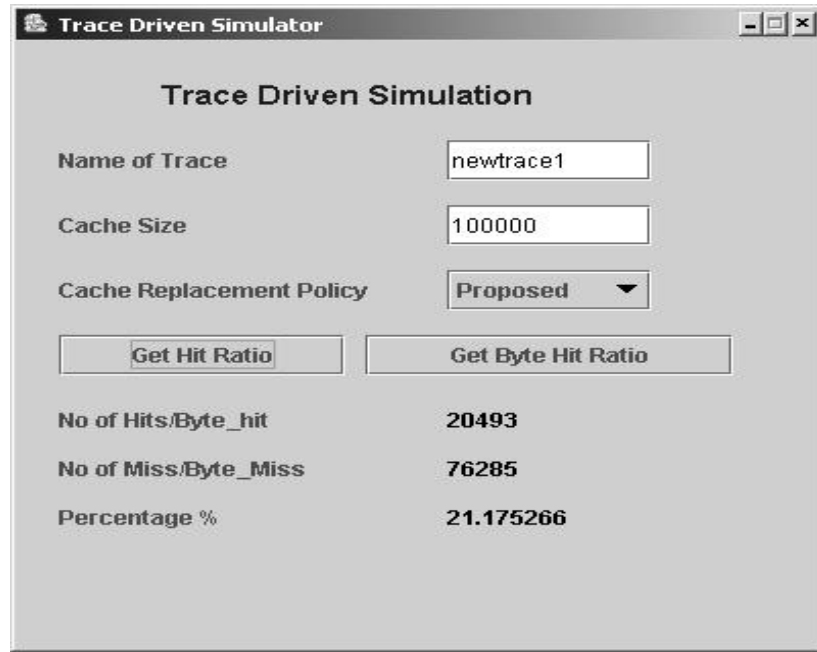
Figure 4.6 Snapshot of the simulator
