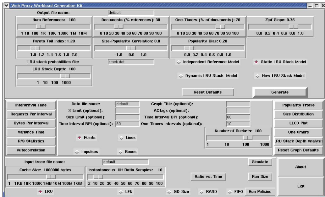
Figure 2.11 Snapshot of the Workload Generator [16]
