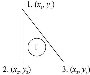
Figure 3-3. The simplest vector field with only 3 vectors.
