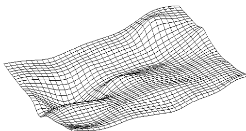
a. The smoothed curl-free potential surface E
