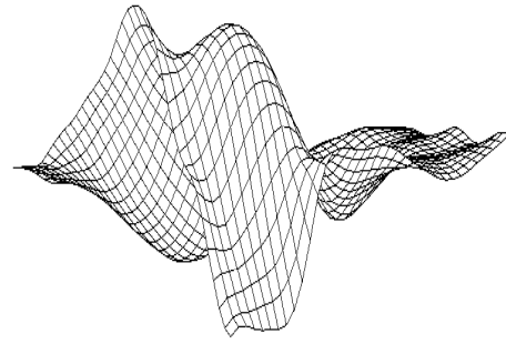
b. The divergence-free potential surface W
