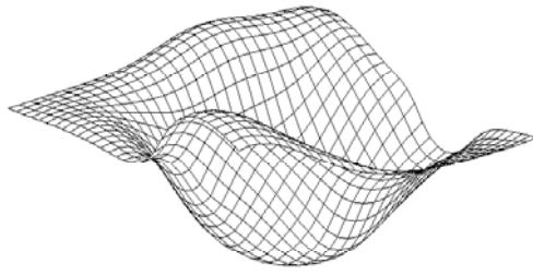
a. The smoothed curl-free potential surface E
