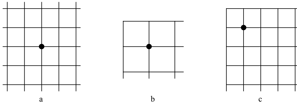
Figure 4-21. Three typical neighborhood configurations for bicubical interpolation. (a) A 5 \times 5 symmetrical neighborhood; (b) A 3 \times 3 symmetrical neighborhood; (c) An asymmetric neighborhood
