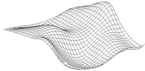
b. The smoothed divergence-free potential surface W
