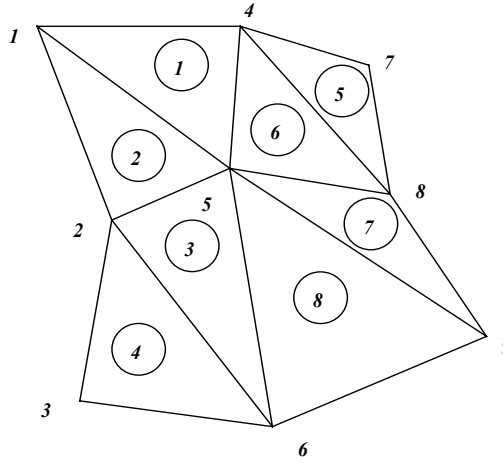
Figure 3-14. Decomposition of a small vector field with 9 vectors using ITG.
