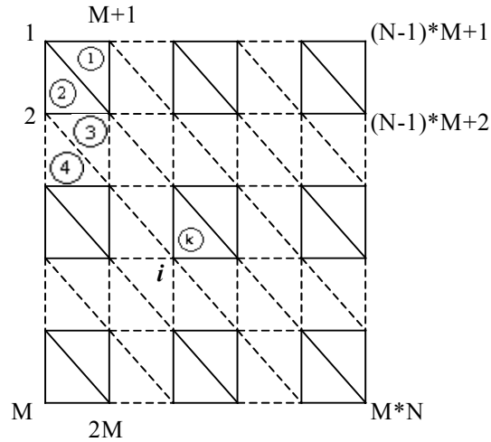
Figure 3-1. Triangulation of the image domain \Omega
