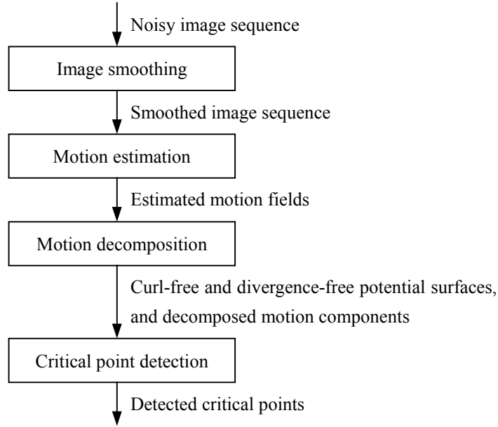
Figure 4-2. Flowchart of the overall framework.
