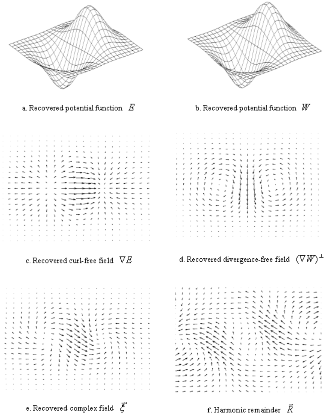
Figure 3-16. Decomposition of a synthetic complex field.
