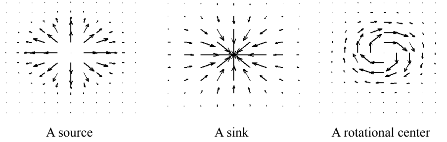
Figure 4-13. Illustration of a source, a sink, and a rotational center.
