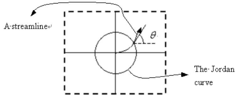
Figure 2-8. Index of a Jordan curve.
