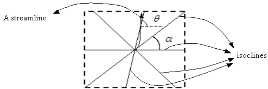
Figure 2-7. Window-clipped isoclines.
