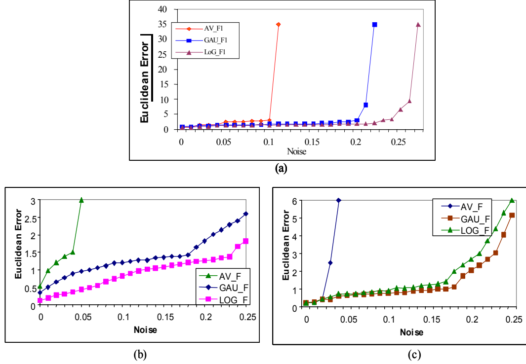
Figure 6.10: Performance of weighting functions for (a) synthetic square sequence (4 features), (b) hybrid workbench sequence, tracking the sharp corners of the computer monitor object (4 features) and (c) hybrid workbench sequence, tracking the chair object (17 features).
