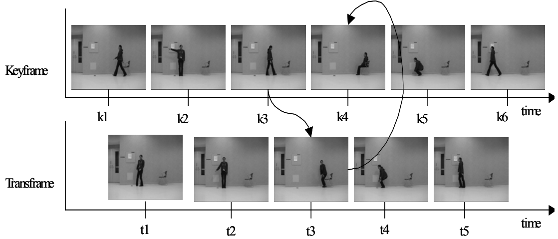
Figure 5.12: Sequential representation of key frames and transitional frames. t3 is one of the transitional frames between k3 depicting ‘walk activity’ and k4 depicting ‘sit activity’.
