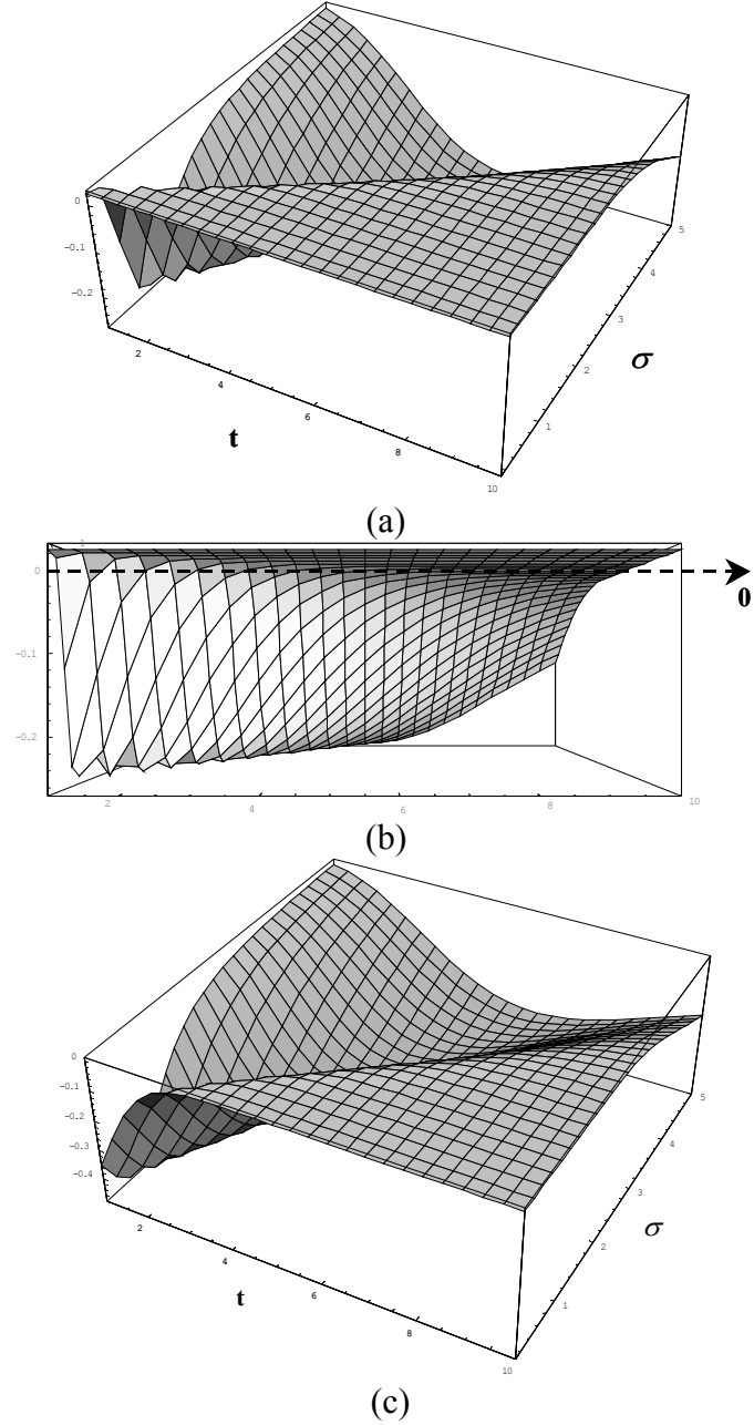
Figure 6.4: Mesh plot Eq. 6.12 for various values of t and \sigma . (a) Eq. 6.12, \sigma_s = 0.01 , (b) Lateral view of (a) highlighting values higher than 0, (c) Eq. 6.12, \sigma_s = 1.0 . Note the negative values corresponding to low values of t and \sigma .
