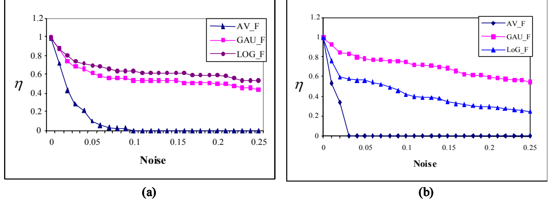
Figure 6.11: Performance of weighting functions with car sequences. (a) Synthetic car sequence, 50 features have been initialized and are being tracked. And (b) Real image car sequence, 50 features have been initialized and are being tracked.
