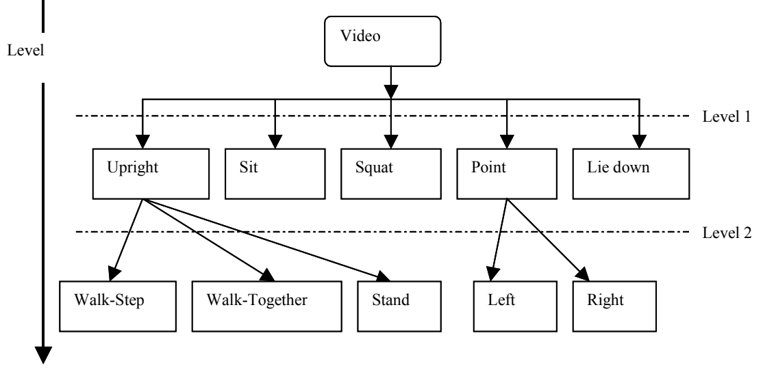
Figure 5.11: Hierarchical clustering levels for higher activity recognition resolution.
