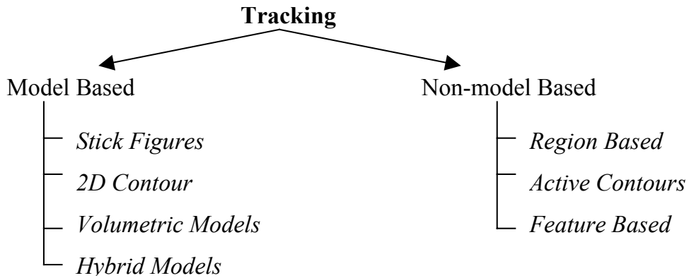
Figure 2.3: Overview of methods for tracking.
