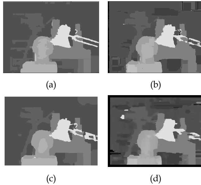
Fig. 4.4 “Tsukuba” depth maps generated by different SDE techniques: (a) the proposed method, (b) FVW [V03], (c) WDP [AD04], (d) RTC [HIG02].
