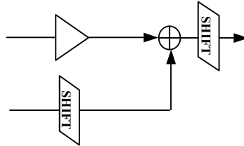
Figure 20. MAC for Asymmetric Wavelet Filters
