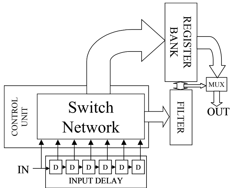
Figure 11. A Systolic Wavelet Architecture [16].
