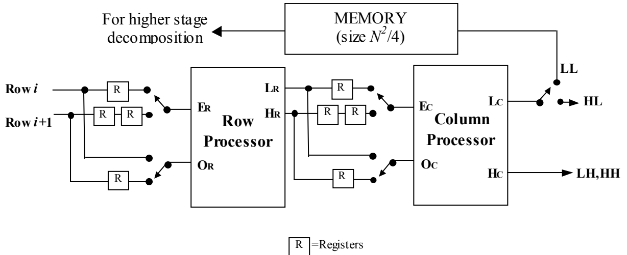
Figure 34. 2-D Dual-scan Architecture
