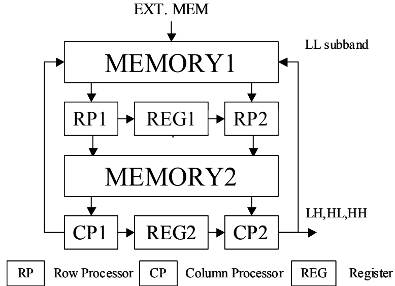
Figure 17. Block Diagram of the 2-D Architecture in [34].
