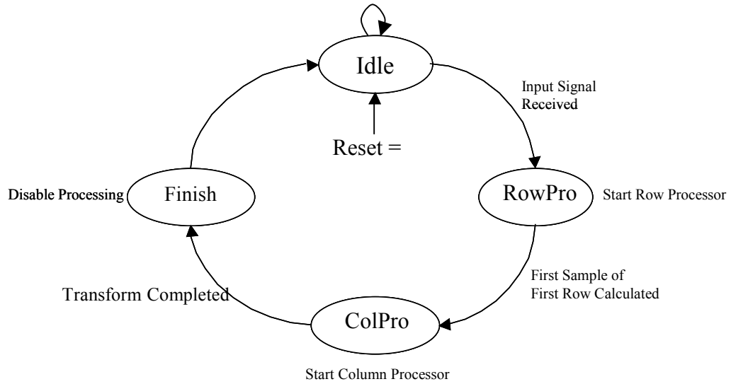
Figure 39. State Transfer Diagram of 2-D DSA
