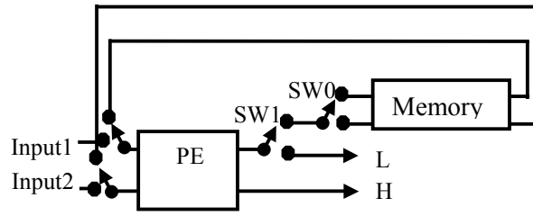
Figure 27. 1-D Dual-scan Architecture
