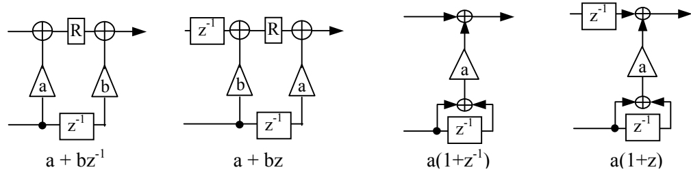
Figure 22. Circuits for the Basic Lifting Steps
