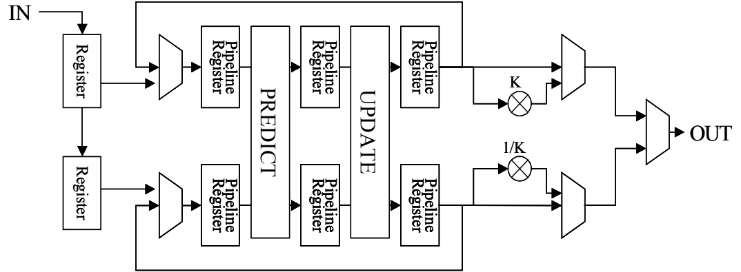
Figure 16. 1-D Folded Architecture [33].
