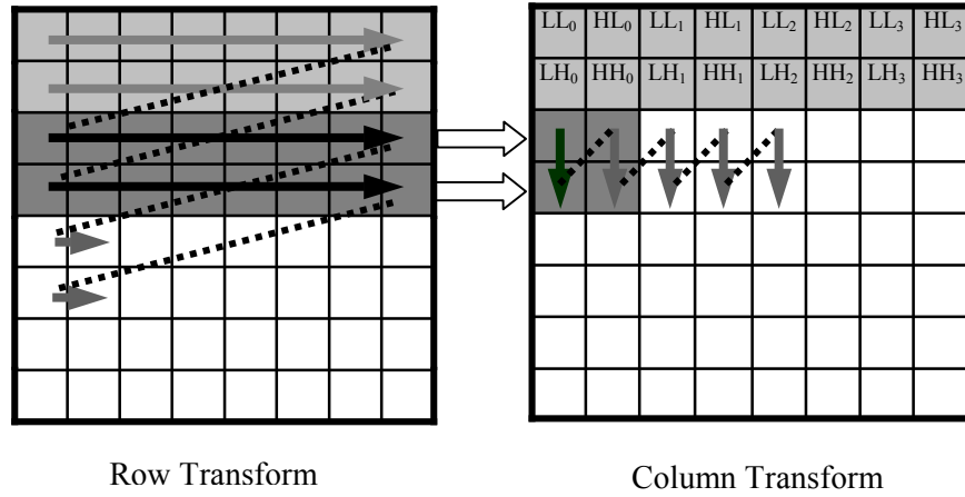
Figure 33. Scan Sequence of the 2-D Dual-scan Architecture
