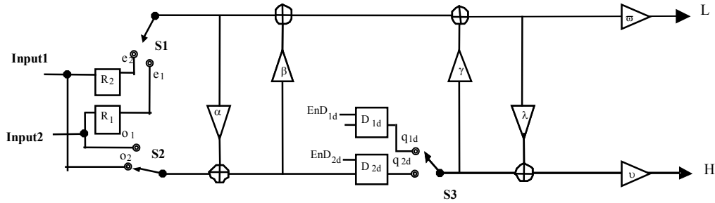
Figure 36. Datapath of 1-D Daub-4 DSA
