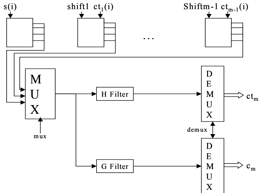
Figure 8. Knowles' Mux Based DWT Architecture [4]
