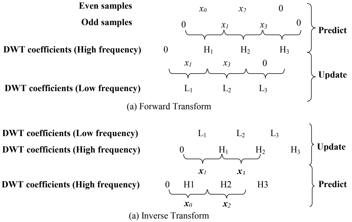
Figure 7. Zero Padding Extension for Short FIR Filters
