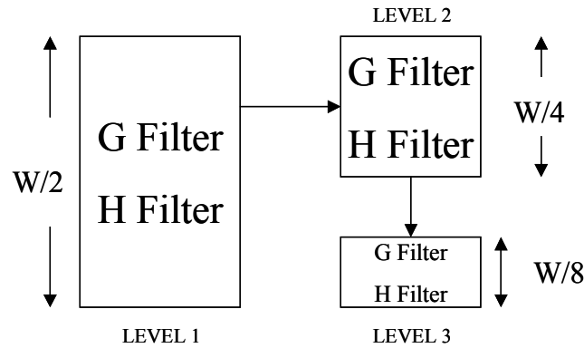
Figure 10. The Diagram of the 1-D Digit-Serial Architecture [8]
