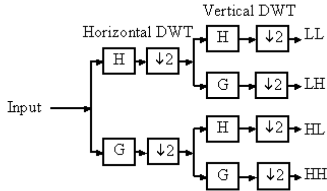
Figure 2. Block Diagram of the 2-D Separable DWT
