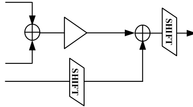
Figure 21. MAC for Symmetric Wavelet Filters
