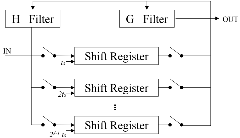
Figure 12. The Parallel Filter Architecture for 1-D DWT [10].
