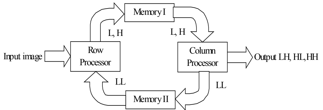
Figure 29. Conventional 2-D Lifting Architecture.
