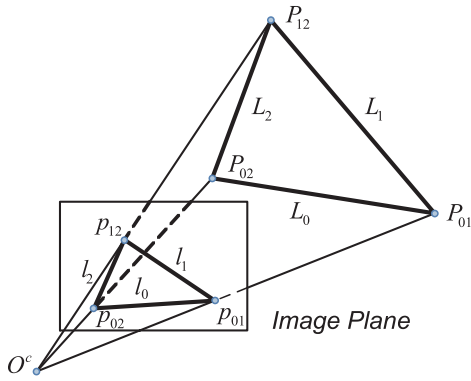
Fig. 2 GEOMETRY OF THE P3P PROBLEM
