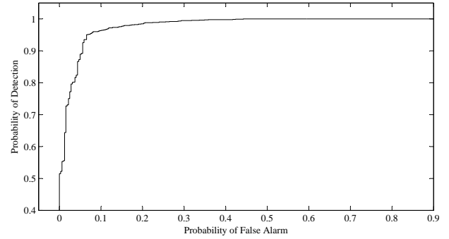
Fig. 7. ROC curve as a function of the OSNR threshold computed from 24 natural photographs.
