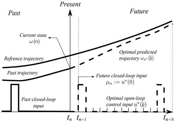
Fig. 9. Illustration of the MPC step at time t_n
