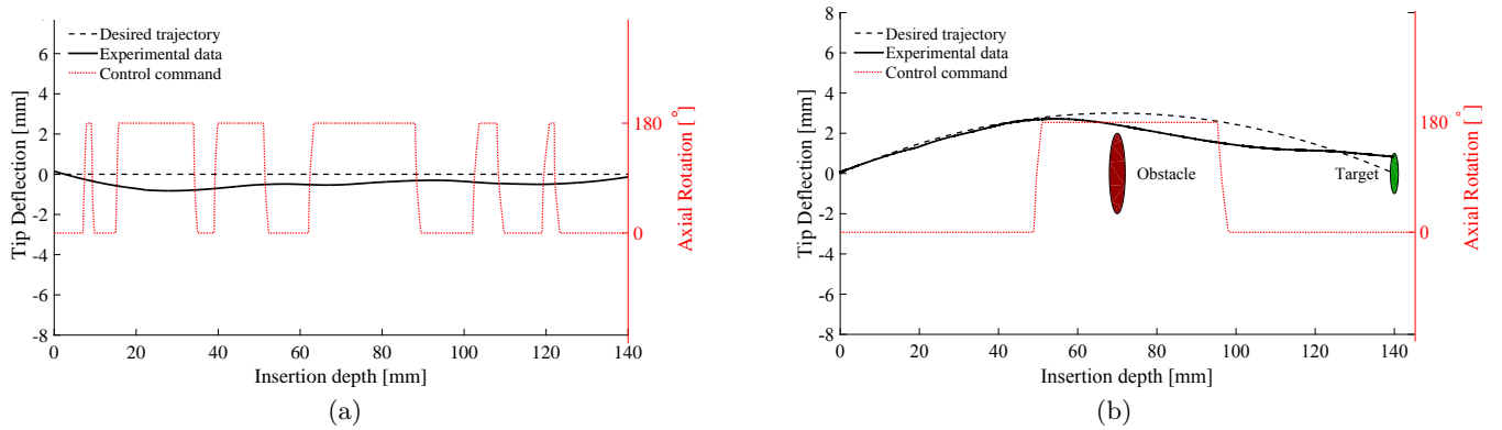
Fig. 13. Representative experimental needle steering results and corresponding controller input command (a) Scenario I–needle steering with the aim of moving on a straight line. (b) Scenario II–needle steering with the aim of manoeuvring around an obstacle.
