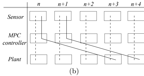
Fig. 10. A schematic of the delay compensation strategy. (a) Block diagram of the time decoupled closed-loop NMPC control with delay compensation. (b) Comparison of scheduling structure between NMPC (dashed line) and NMPC with delay compensation with t_{max} = 3 * \text{sampling time} (solid line)
