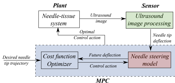
Fig. 2. Scheme of the MPC closed-loop components.
