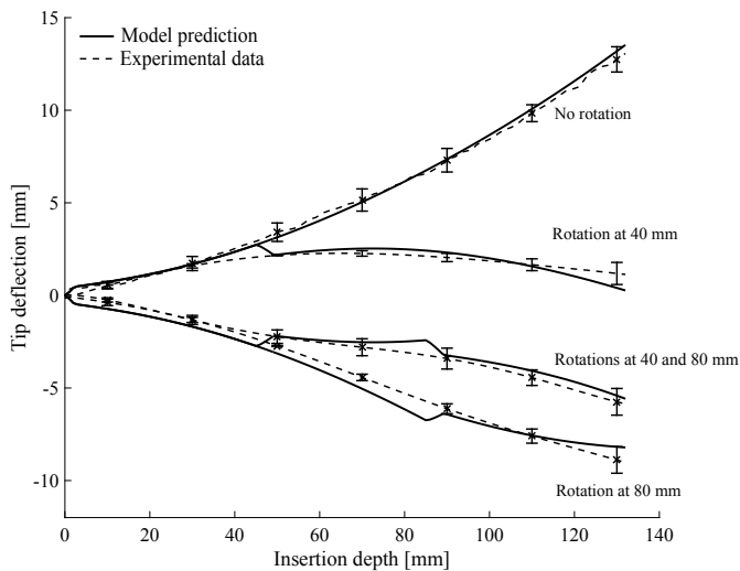
Fig. 12. A comparison of experimentally-obtained needle tip deflections and the corresponding model predictions for needle insertion at constant velocity of 5 mm/sec with and without axial axial rotations. Error bars denote standard deviation of experimental data.
