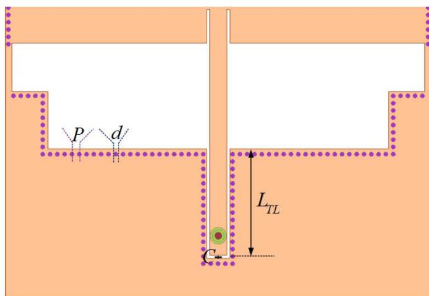
Fig. 2. Position of coaxial feed C .
