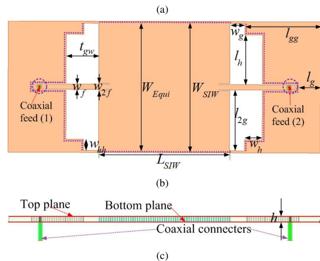
Fig. 1. The proposed transition: (a) Stereoscopic view, (b) Top view, (c) Cross-sectional view.
