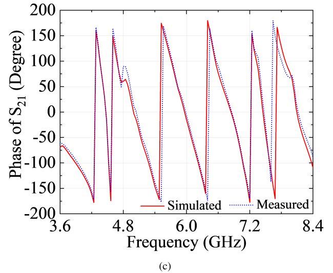
Fig. 7. Simulated and measured results: (a) |S_{11}| and |S_{21}| , (b) Total loss, and (c) Phase of S_{21} .
