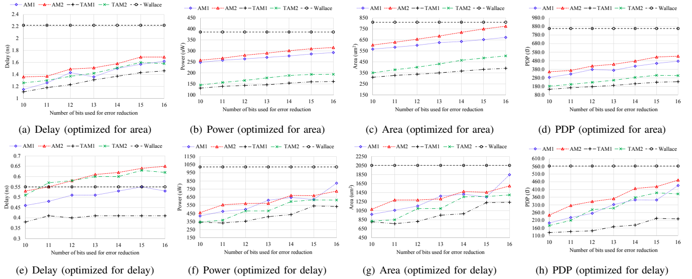
Fig. 10. Delay, power and area comparisons of proposed 16 \times 16 approximate and the optimized Wallace multipliers. “Wallace” indicates the accurate 16 \times 16 Wallace multiplier, and the X-axis is not applicable for it.
