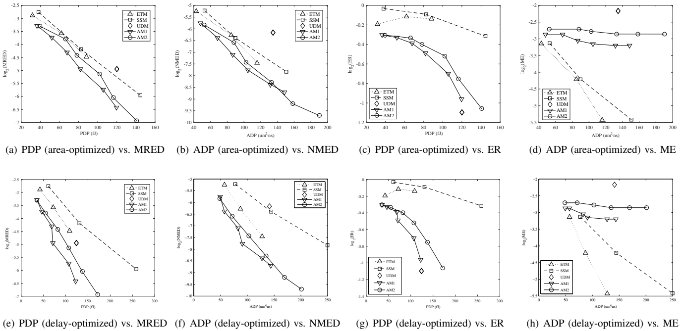
Fig. 11. Comparison of accuracy and hardware among five approximate 8 \times 8 multipliers. The number of MSBs used for error reduction for AM1 and AM2 ranges from 4 to 9 from left to right. The width of the accurate multiplier for ETM and SSM ranges from 4 to 6 from left to right.
