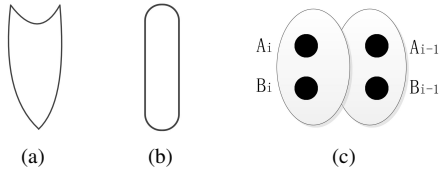
Fig. 2. Symbols for (a) an OR gate, (b) an full adder or a half adder and (c) an approximate adder cell
