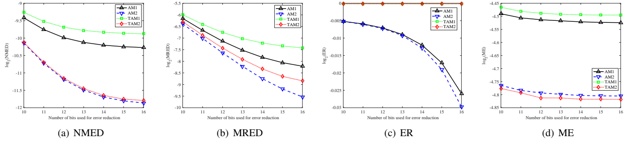
Fig. 7. Accuracy comparison of the approximate 16 \times 16 multipliers vs. the number of bits used for error reduction.
