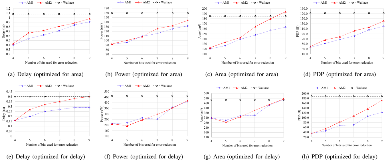
Fig. 9. Delay, power and area comparisons of proposed 8 \times 8 approximate and Wallace multipliers. “Wallace” indicates the accurate 8 \times 8 Wallace multiplier, and the X-axis is not applicable for it.
