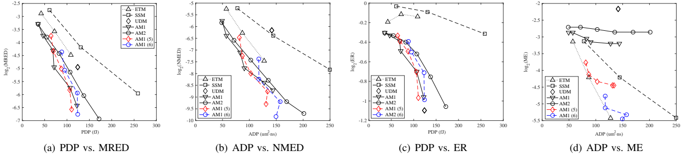
Fig. 13. Comparison of accuracy and hardware (delay-optimized) of improved 8 \times 8 AM1 with other designs. The number of MSBs used for error reduction for AM1 and AM2 ranges from 4 to 9, and the width of the accurate multiplier for ETM and SSM is from 4 to 6, from left to right. AM1 (5) and AM1 (6) are AM1's with 5 and 6 MSBs of errors that are correctly accumulated. Thus, the number of MSBs used for error reduction for AM1 (5) is from 5 to 9, and it is from 6 to 9 for AM1 (6).
