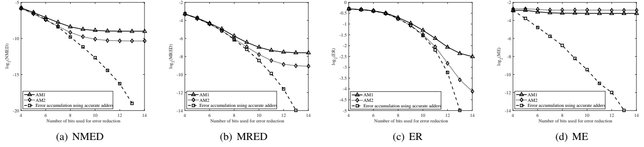
Fig. 6. Accuracy comparison of the approximate 8 \times 8 multiplier using approximate and exact error accumulation vs. different number of bits for error reduction.
