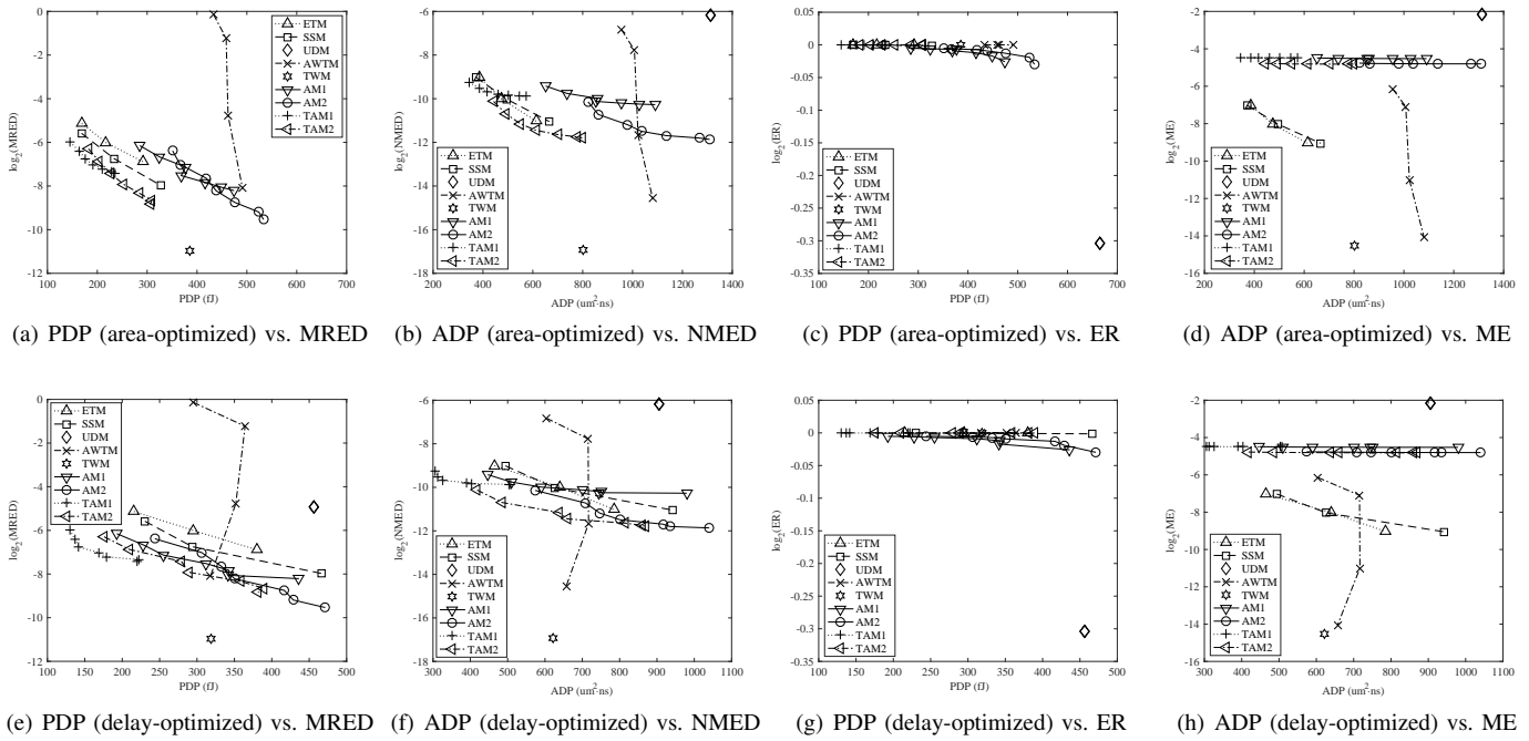
Fig. 12. Comparison of accuracy and hardware of approximate 16 \times 16 multipliers. The width of the accurate multiplier for ETM and SSM ranges from 8 to 10 from left to right. The parameter for AWTM is the mode number (1 to 4) from left to right.
