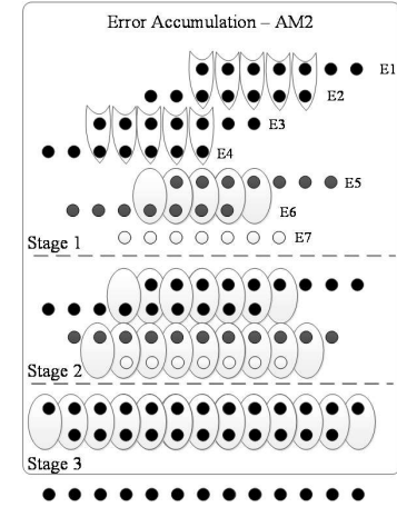
Fig. 4. Error accumulation tree for AM2. ●: an error bit generated at the first stage; ●: an error bit generated at the second stage; ○: an error bit generated at the last stage.
