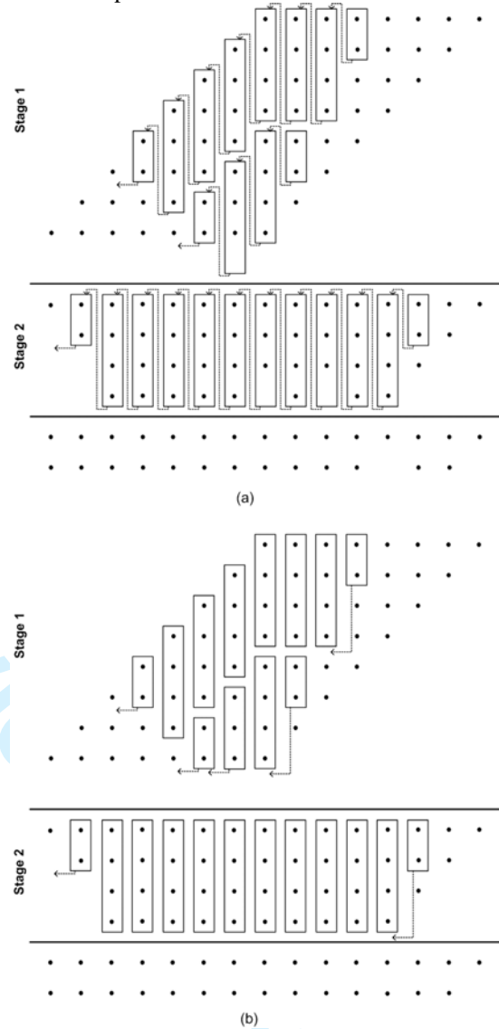
Figure 9. Reduction circuitry of an 8 \times 8 Dadda multiplier, (a) using Design 1 compressors, (b) using Design 2 compressors
