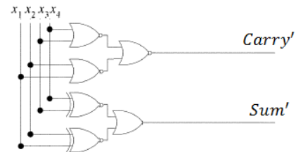
Figure 8. Gate level implementation of Design 2
