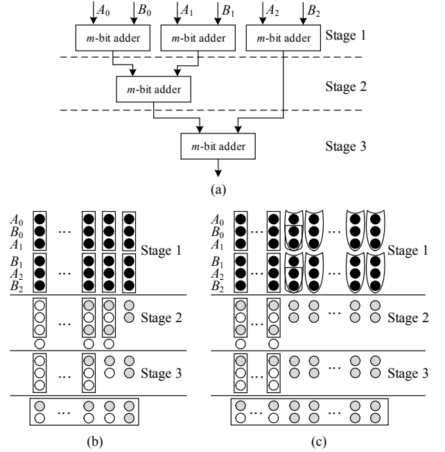
Fig. 10. Accumulation of partial products by (a) a traditional adder tree, (b) a Wallace tree and (c) an approximate Wallace tree. \bullet : an input bit; \odot : the sum bit from the previous layer; \circ : the carry bit from the previous layer; \square : a full adder; \mathcal{D} : an OR gate; \mathcal{D} : an AND gate.
