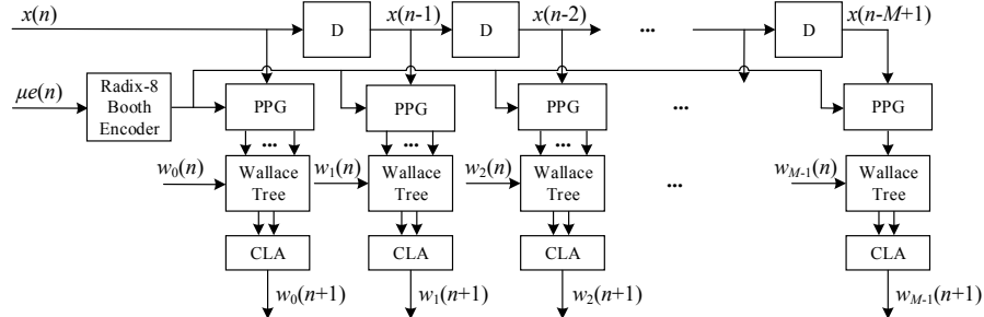
Fig. 8. Proposed weight update scheme. PPG: the partial product generator; CLA: the m -bit carry lookahead adder.
