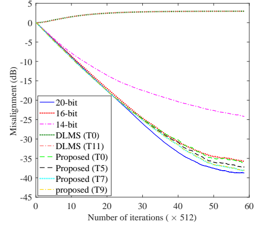
Fig. 16. Learning curves in the normalized misalignment of 128-tap FIR adaptive filter designs.
