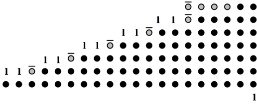
Fig. 6. Partial product tree of an approximate 20 \times 20 radix-8 Booth multiplier with truncation. ●: a partial product; ●: a sign bit; ○: an inverted sign bit.
