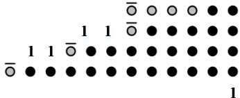
Fig. 7. Partial product tree of an approximate 12 \times 20 radix-8 Booth multiplier with truncation. ●: a partial product; ●: a sign bit; ○: an inverted sign bit.
