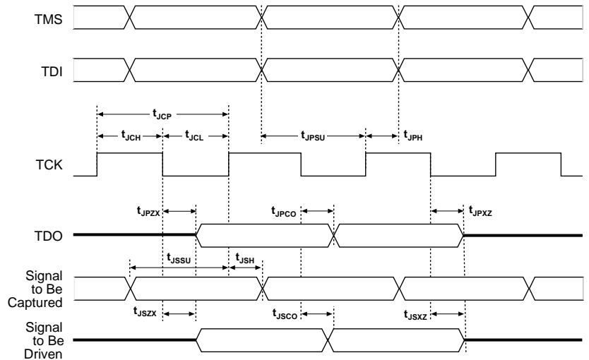
Figure 17. JTAG Waveforms
