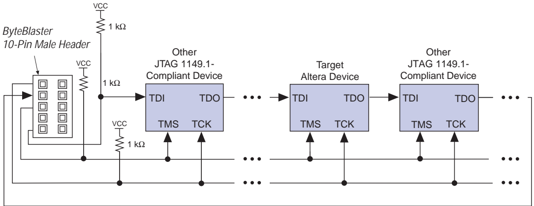
Figure 11. JTAG-Chain Device Programming &amp; Configuration with the ByteBlaster Cable
