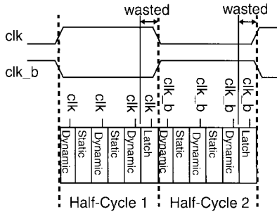
Fig. 1. Domino pipeline with ideal clocks.
