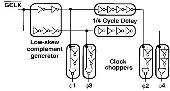
Fig. 12. Four-phase clock generation.
