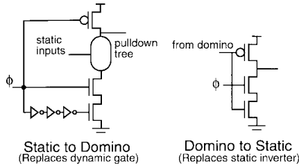
Fig. 14. Domino/static interfaces.
