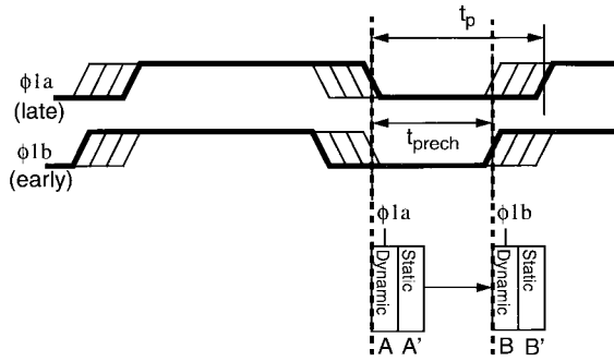
Fig. 5. Precharge time constraint.
