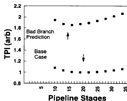
Fig. 7 shows the effect of changing branch prediction on the optimal pipeline depth.
