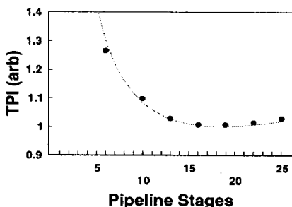
Fig. 5 is a direct comparison of the simulation (data points) and the theory (solid curve) for a particular workload. The TPI numbers are scaled to the minimum point.
