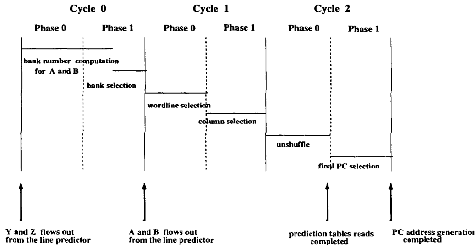
Figure 3. Flow of the branch predictor tables read access
