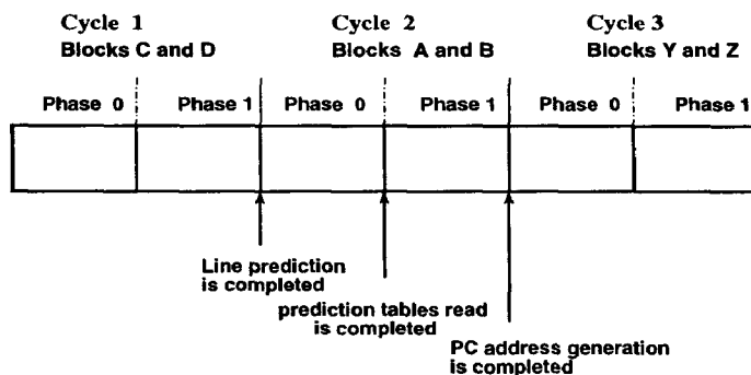
Figure 1. PC address generation pipeline
