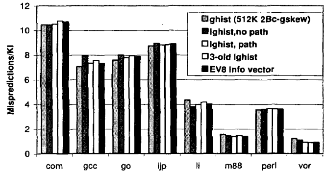
Figure 7. Impact of the information vector on branch prediction accuracy
