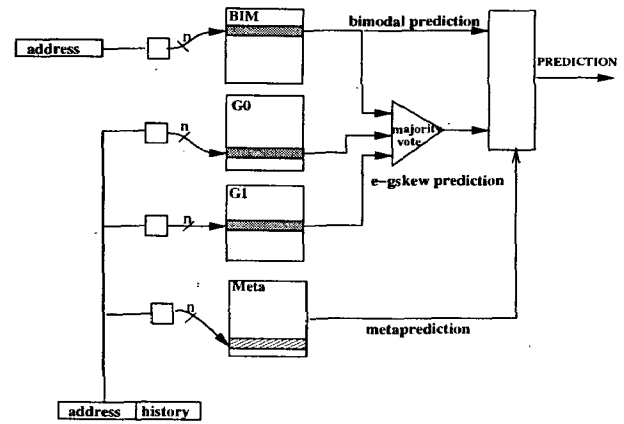
Figure 2. The 2Bc-gskew predictor
