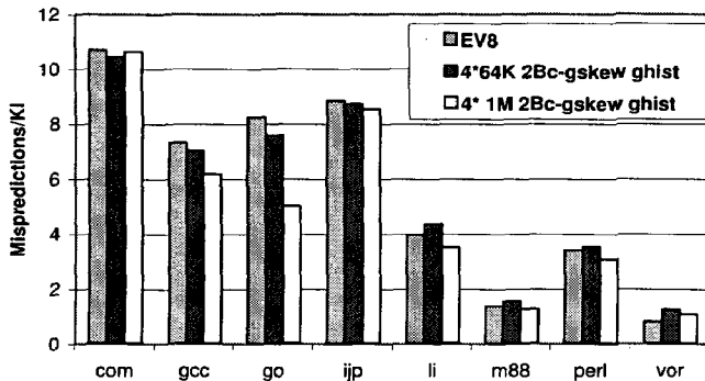
Figure 10. Limits of using global history
