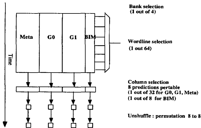
Figure 4. Reading the branch prediction tables
