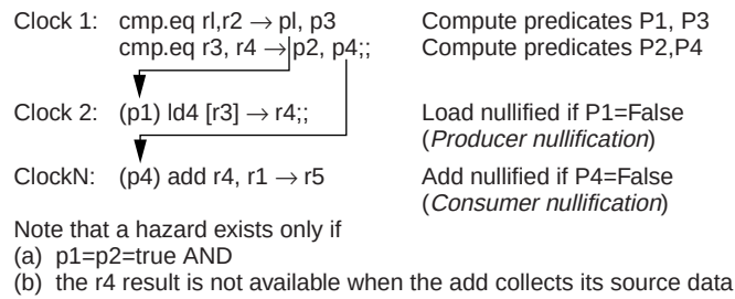
Figure 7. Predicated producer-consumer dependencies.
