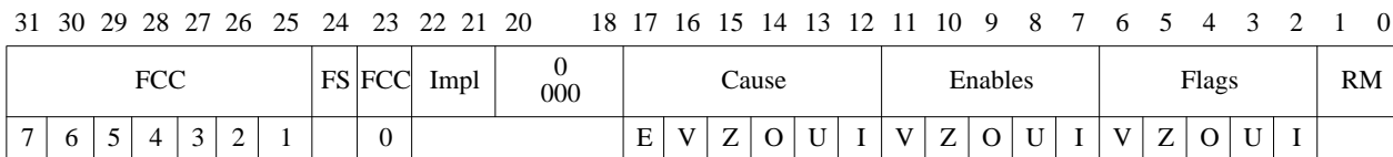
Figure 5-12 FCSR Register Format
