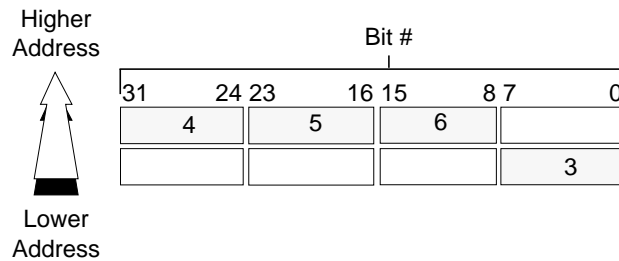
Figure 2-13 Big-Endian Misaligned Word Addressing
