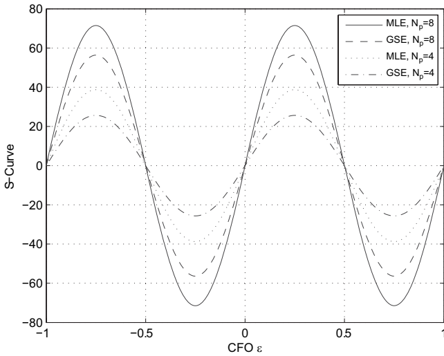
Fig. 6. S-curve for a QPSK OFDM system with N = 64 , N_v = 12 and SNR = 10 dB.
