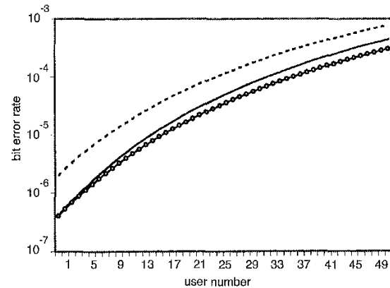
Fig. 1 Simulation result over Rayleigh fading channels
