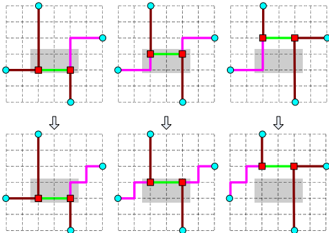
Fig.9. Different routing solutions for one POWV
