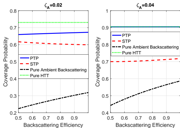
Fig. 9. Coverage probability as a function of backscattering efficiency.
