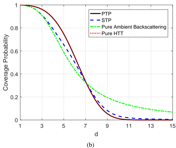
Fig. 11. Comparison of coverage probabilities as a function of d (unit: m). ((a) \zeta_A = 0.02 , \xi = 0.1 , (b) \zeta_A = 0.04 , \xi = 0.6 )
