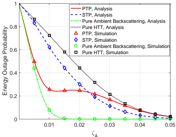
Fig. 5. Comparison of energy outage probabilities. ( \alpha = -1 )
