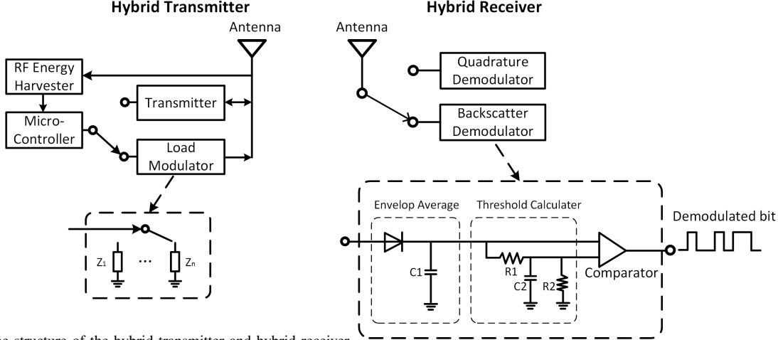
Fig. 1. The structure of the hybrid transmitter and hybrid receiver.
