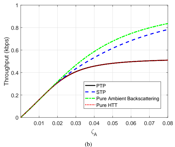
Fig. 12. Comparison of average throughput as a function of \zeta_A . ((a) d = 5 , \xi = 0.2 , (b) d = 5 , \xi = 0.8 )
