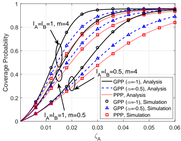
Fig. 6. C_{PTP} as a function of \zeta_A .
