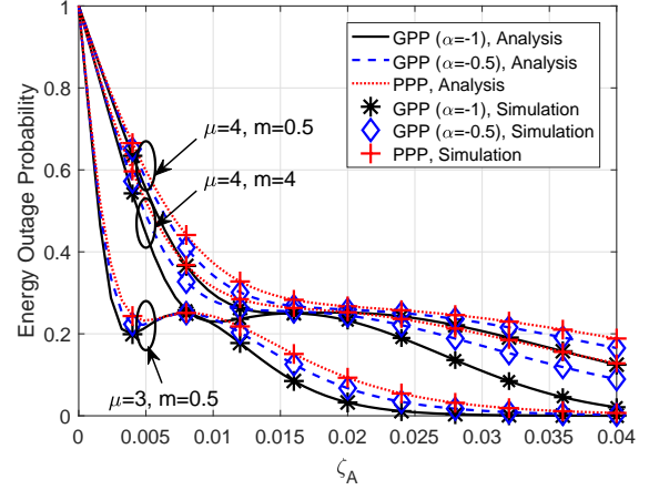
Fig. 3. \mathcal{O}_{\text{PTP}} as a function of \zeta_A .
