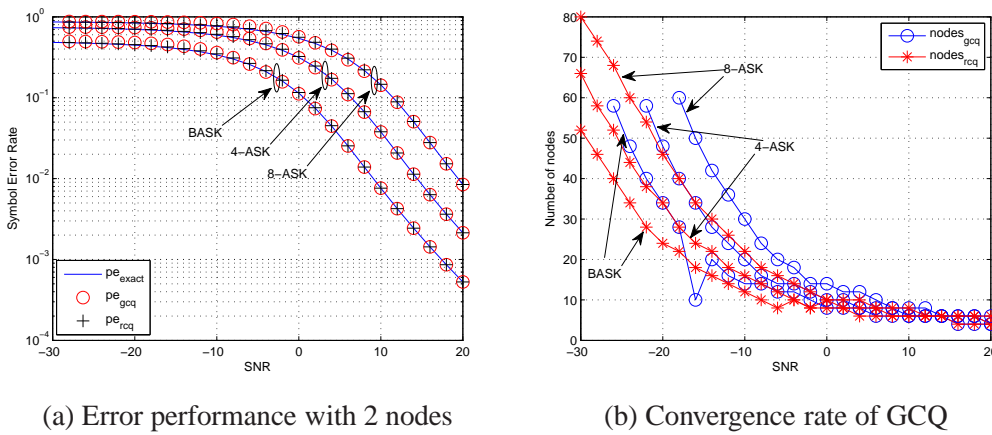
Figure 3.17: Coherent Detection of M -ary ASK ( M = 2, 4, 8 ) in Rician fading ( K = 3 ).
