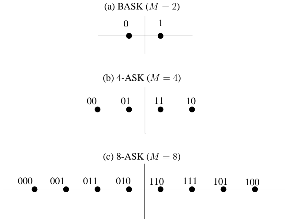
Figure 2.2: ASK Constellation [1]
