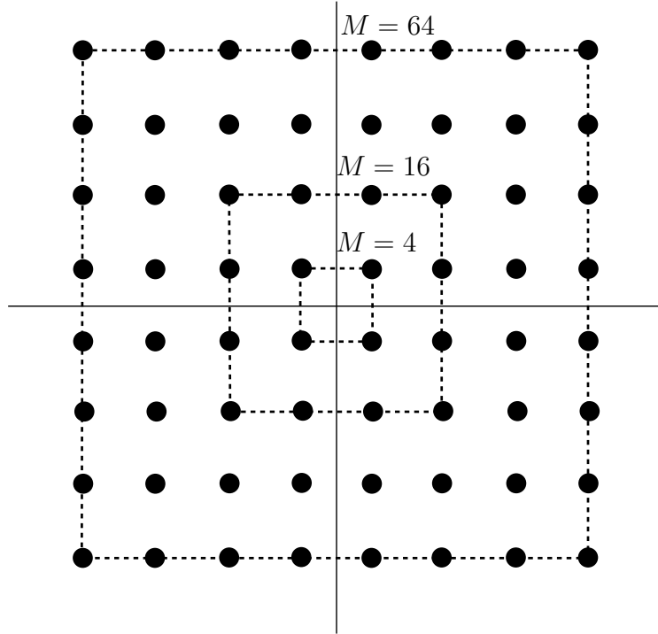
Figure 2.4: QAM Constellation [1]
